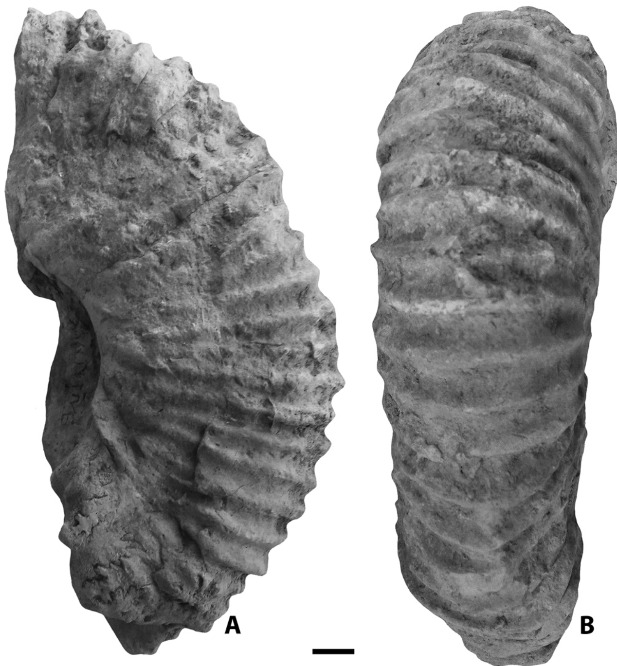
Plate 1: Lateral view (A) and ventral view (B) of Cheloniceras sp. (MHNUL 22797/0006), lowermost Cardium Beds, Kanat Bakich. Scale bar = 1 cm.
