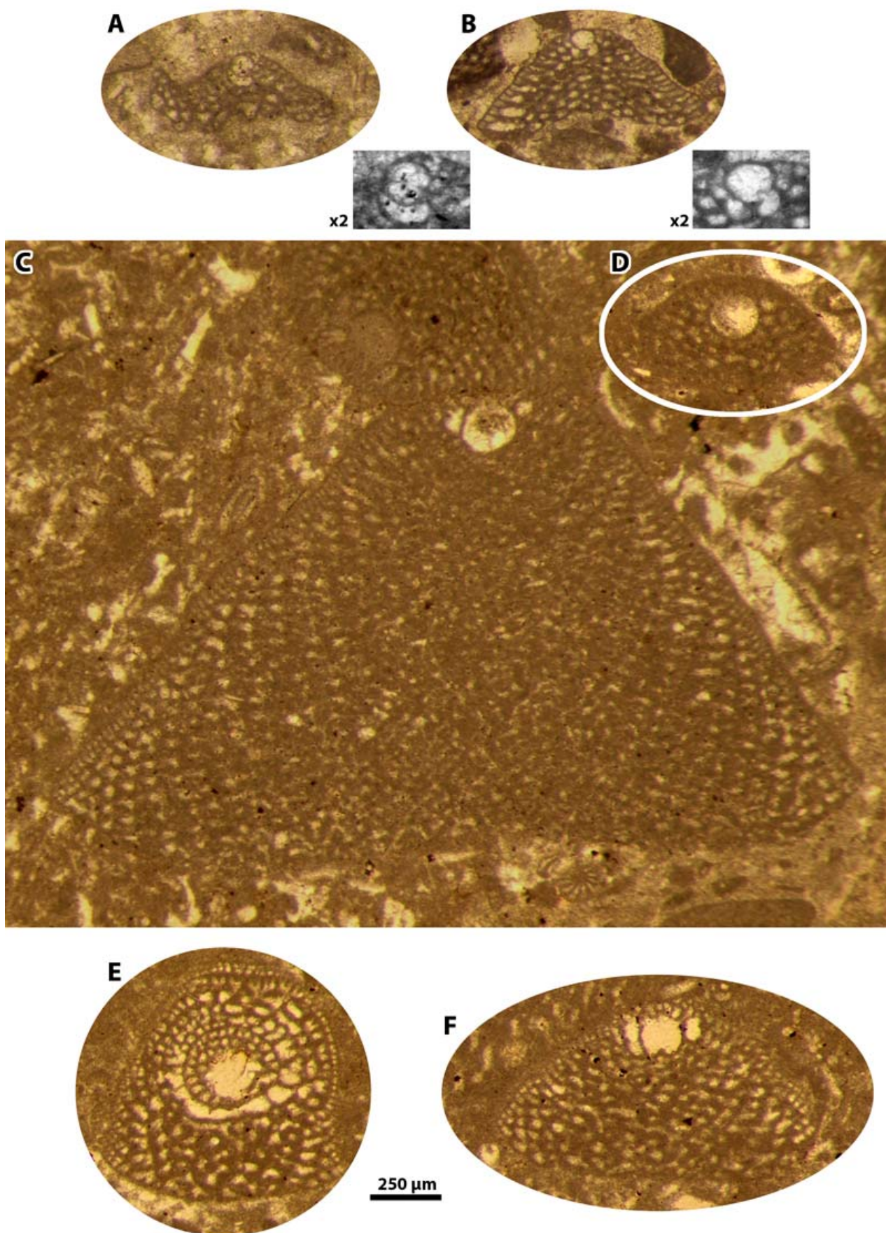
Figure 8: A-B: Slightly oblique and axial sections of Praeorbitolina cormyi SCHROEDER, 1964, from the "Orbitolina Beds", directly above the Jezzian section at Jezzine, thin-section JEZh; C-D: Axial and slightly oblique sections of Palorbitolina lenticularis (BLUMENBACH, 1805) from Jezzian strata, East Ain Dara, thin-section EAD38; E-F: Tangential and axial sections of Palorbitolina lenticularis (BLUMENBACH, 1805) from Jezzian strata, East Ain Dara, thin-section EAD 68; scale bar = 250 µm (or 500 µm for "x2").
