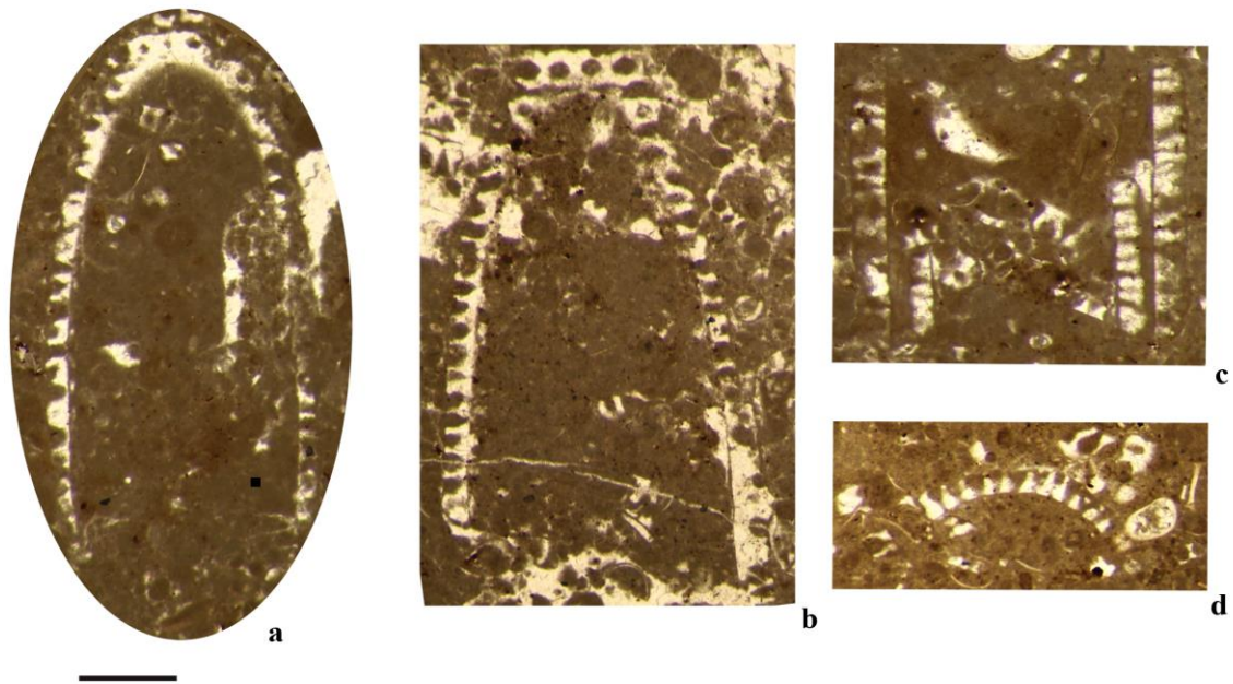
Fig. 11 a-d Harlanjohnsonella annulata Elliott in Granier & Deloffre, 1993, non 1968; topotypic material (Collection Deloffre, Leg. Radoičić); a Oblique section; b Oblique section; c Longitudinal section; d Fragment in a transverse section. Scale bar = 0.5 mm.
