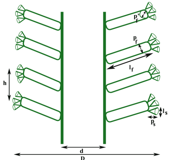
Fig. 6 Schematic reconstruction of Triploporella steinmannii Barattolo, 1983.
